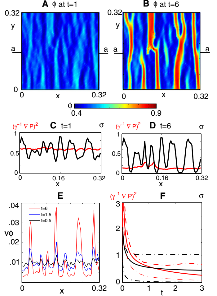
Fig. 2: (Color online) Numerical solution to eqs. (1)–(7) with a steady specific discharge q = q_0 prescribed at the lower boundary y = 0 , and constant pressure at the upper boundary y = 0.32 . (A) Spatial distribution of porosity \phi at t = 1 and (B) at t = 6 . (C) (\gamma^{-1}\nabla p)^2 (red) and \sigma (black) are plotted along a-a (at y = 0.16 ) at t = 1 and (D) at t = 6 corresponding to the panels above. Erosion occurs where (\gamma^{-1}\nabla p)^2 > \sigma . At early times, this occurs at several locations. As erosion progresses, the pressure gradient drops, heterogeneity in \sigma increases, and erosion is limited only to the channels. (E) The flux in the y -direction, v(\phi_g + \phi_l) plotted at section a-a at t = 0.5 (black), t = 1.5 (red), and at t = 6 (blue). As the flux increases in eroded regions, it decreases in non-channelized regions. (F) Domain-averaged time evolution of the scaled pressure gradient squared (solid red line) and erosion threshold (solid black line), with one standard deviation plus or minus (dash-dotted lines) indicated. Initially, the area-averaged (\gamma^{-1}\nabla p)^2 > \sigma , but as erosion progresses, the pressure gradient decreases, (\gamma^{-1}\nabla p)^2 < \sigma , and erosion no longer occurs, except in a few places.
