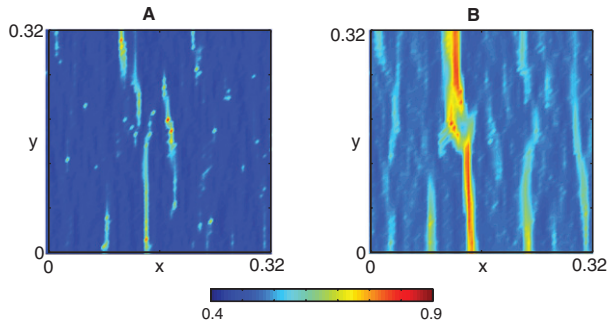
Fig. 5: (Color online) The evolution of the porosity is sensitive to the functional form of the erosion threshold \sigma . Here the final distribution of porosity \phi is shown for other choices of \sigma . (A) \sigma = \bar{\phi}_s , (B) \sigma = \bar{\phi}_s^2 . These results can be compared with fig. 1, where \sigma = 0.5(\tanh(2\pi(\bar{\phi}_s - 0.6)) + 1) (subtracting 0.6 instead of 0.5 provides a slight asymmetry to the tanh profile).
